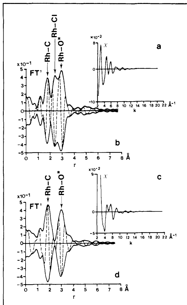
Figure 6. The dimer {Rh(CO) 2 Cl} 2 : (a) the normalized primary EXAFS data of the rhodium K-edge at 77 K; (b) the associated k^2 -weighted Fourier transform ( \Delta k = 2.44 – 12.6 \text{ \AA}^{-1} , Rh–O phase shift corrected) [solid line = |FT'| , dotted line = \text{Im}FT' ]; (c) the difference between the normalized EXAFS data and the calculated contribution of the nearest neighbor chlorine atoms; (d) the k^2 -weighted Fourier transform of the difference signal ( \Delta k = 3.3 – 10 \text{ \AA}^{-1} , Rh–O phase shift corrected) [solid line = |FT'| , dotted line = \text{Im}FT' ].
