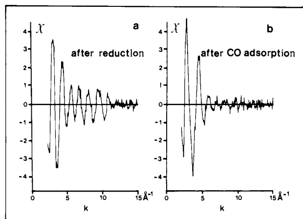
Figure 3. The primary EXAFS data of the rhodium K-edge at 77 K of the 0.57 wt % Rh/ \gamma -Al 2 O 3 catalyst after (a) reduction at 593 K (100 kPa of H 2 ) and (b) CO adsorption at room temperature (100 kPa of CO).
