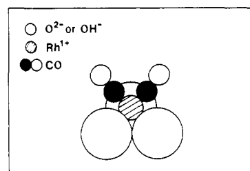
Figure 11. Possible structure of \text{Rh}(\text{CO})_2 species attached to the \gamma\text{-Al}_2\text{O}_3 support after CO admission at 298 K.
